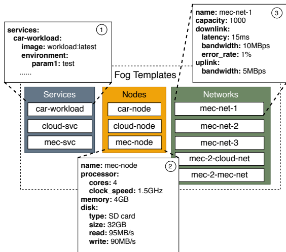
Fig. 4: Templates of Smart Transportation Scenario
