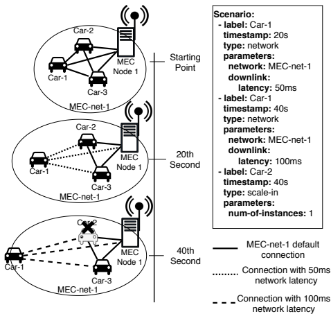
Fig. 6: Moving Node & Fault Scenario
