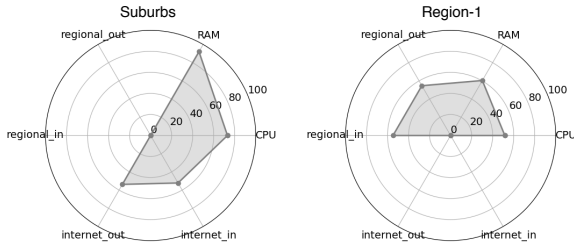
Fig. 15: Fog node profiling when moving between regions
