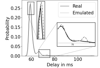
Fig. 10: Latency Distribution
