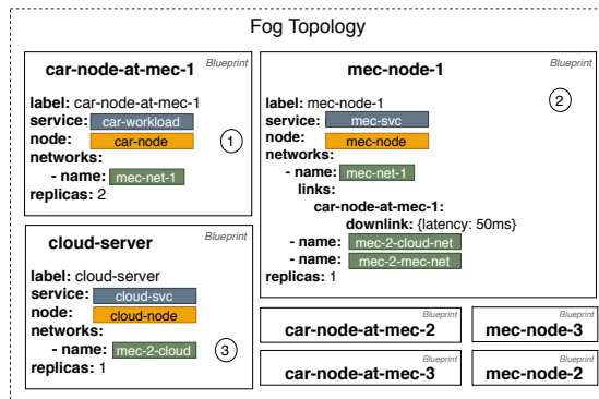
Fig. 5: Examples of Fog Topology Model
