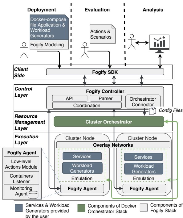
Fig. 2: A High-Level Overview of the Fogify Emulator
