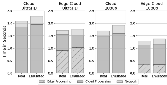
Fig. 13: Application in different deployments
