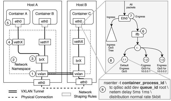
Fig. 7: Low-level network shaping of Fogify
