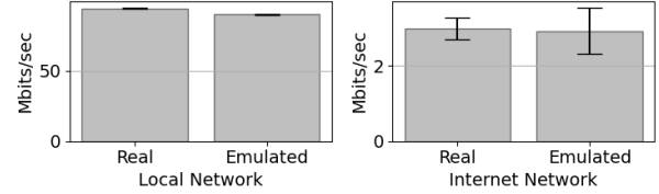
Fig. 11: Network Link Bandwidth Realism
