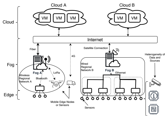
Fig. 1: High-Level Overview of an Exemplary Fog Topology
