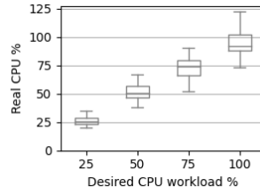
Fig. 9: Compute Realism
