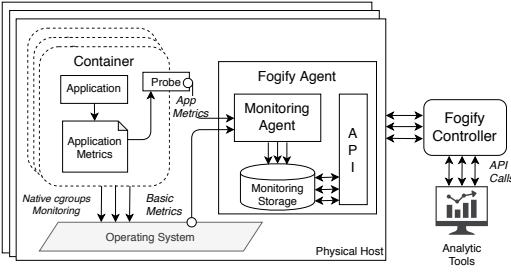
Fig. 8: Monitoring System Overview
