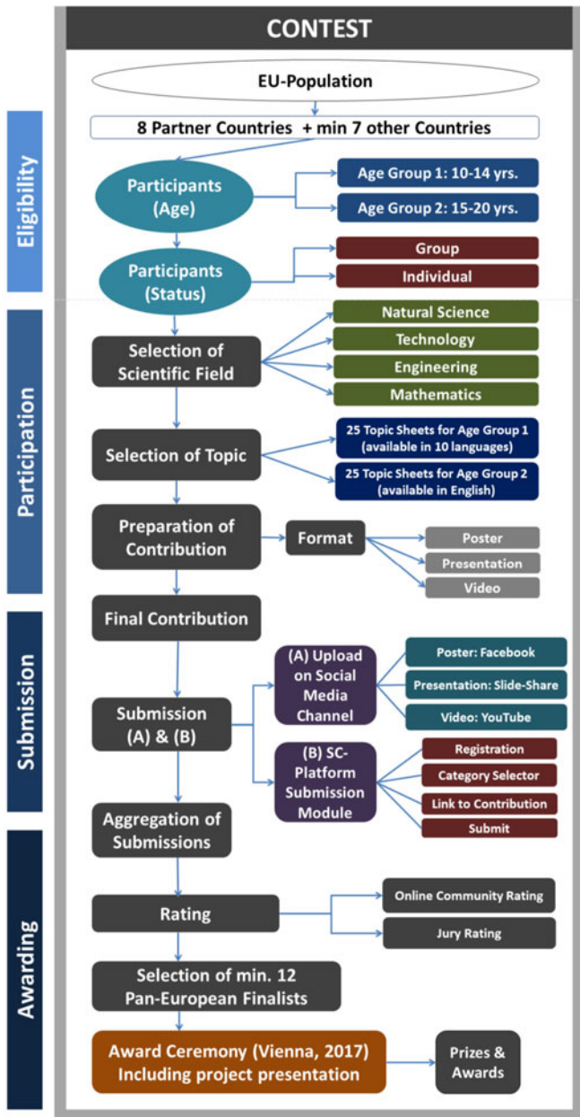
Fig. 1. SciChallenge concept.
